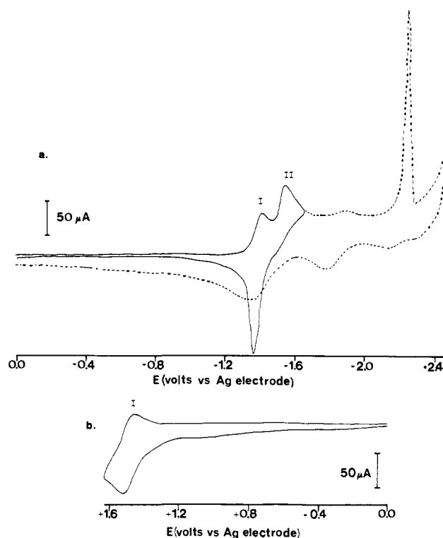
Figure 4. Cyclic voltammogram of 1 mM Ru(o-phen) 3 (ClO 4 ) 2 /CH 3 CN/0.1 M TBABF 4 at a Pt disk microelectrode: (a) (—) scan from 0.0 to -2.5 V, scan rate = 200 mV/sec; (---), scan from -2.5 V to 0.0, scan rate = 200 mV/sec; (b) scan from 0.0 to +1.65 V, scan rate = 200 mV/sec.
