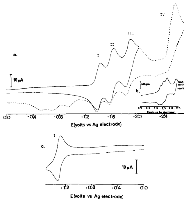
Figure 1. Cyclic voltammogram of 1 mM \text{Ru}(\text{bipy})_3(\text{ClO}_4)_2/\text{CH}_3\text{CN}/0.1 M \text{TBABF}_4 at a Pt disk microelectrode: (a) scan from 0.0 to -2.6 V, scan rate = 200 mV/sec; (b) scan as a, scan rate = 100 V/sec; (c) scan from 0.0 to +1.4 V, scan rate = 200 mV/sec.
